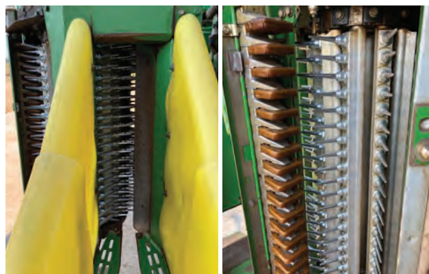
The spindle picker uses spindles, doffers and pads to pick cotton from bolls. © René van der Sluijs
