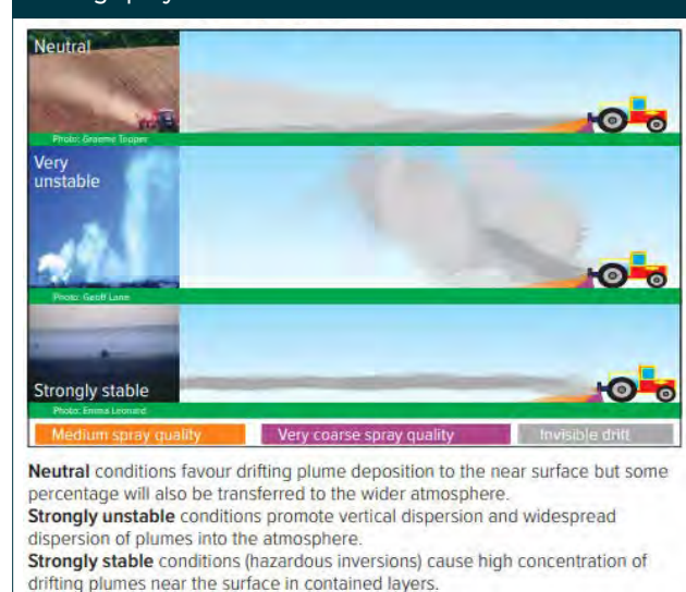
FIGURE 18.4 Three common states of atmospheric stability and their relationship to spray application and drifting sprays.
