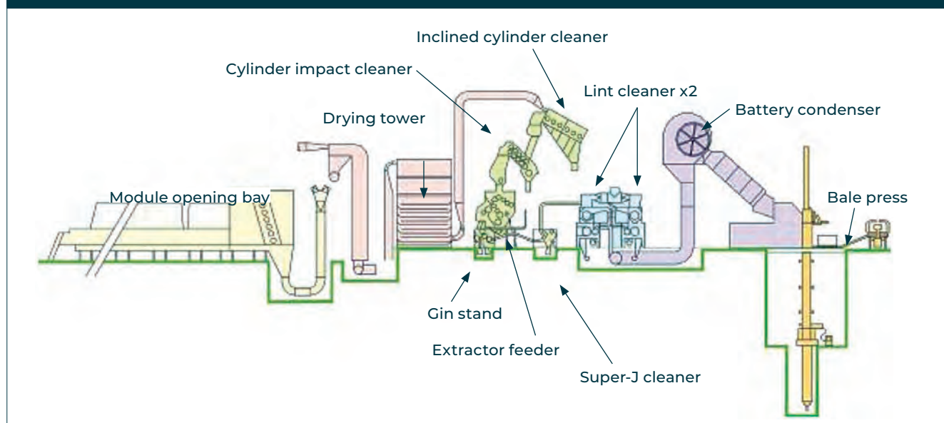
FIGURE 22.1 Gin flow diagram shows cross-sections of machines used in a modern gin to process spindle-harvested cotton.
