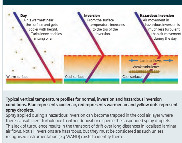
FIGURE 18.3 What is a hazardous inversion?
