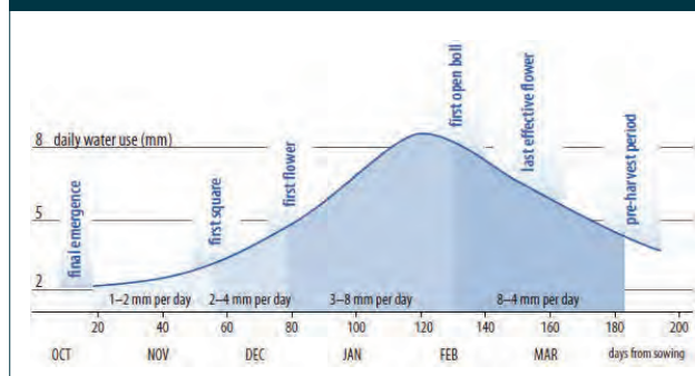
FIGURE 5.2 Nominal seasonal daily water use (mm/day) for cotton production. (Source: WATERpak Figure 2.1.3)
