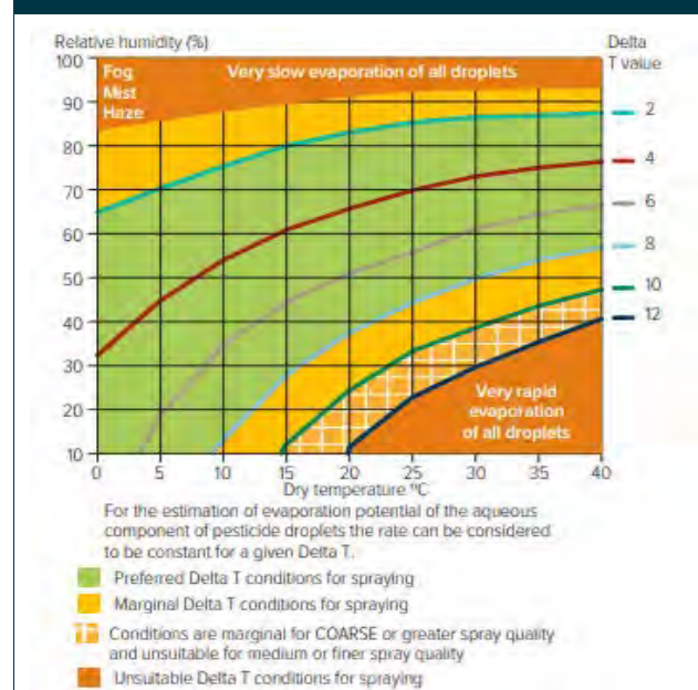
FIGURE 18.1 Delta T is used to indicate evaporation rate and droplet survival. Spraying operations are best conducted when Delta T is between 2 and 8.
